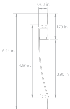
WALL ACCENT 4 in.
