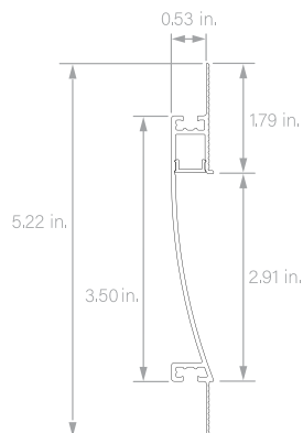
WALL ACCENT 3 in. *
