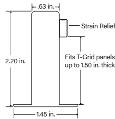
Any T-Grid - Linear
